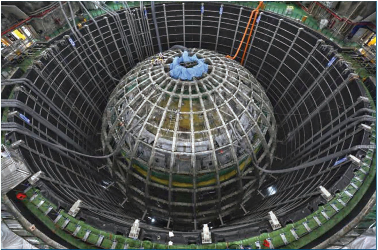
Fig. 17. Current status of the JUNO detector assembly
