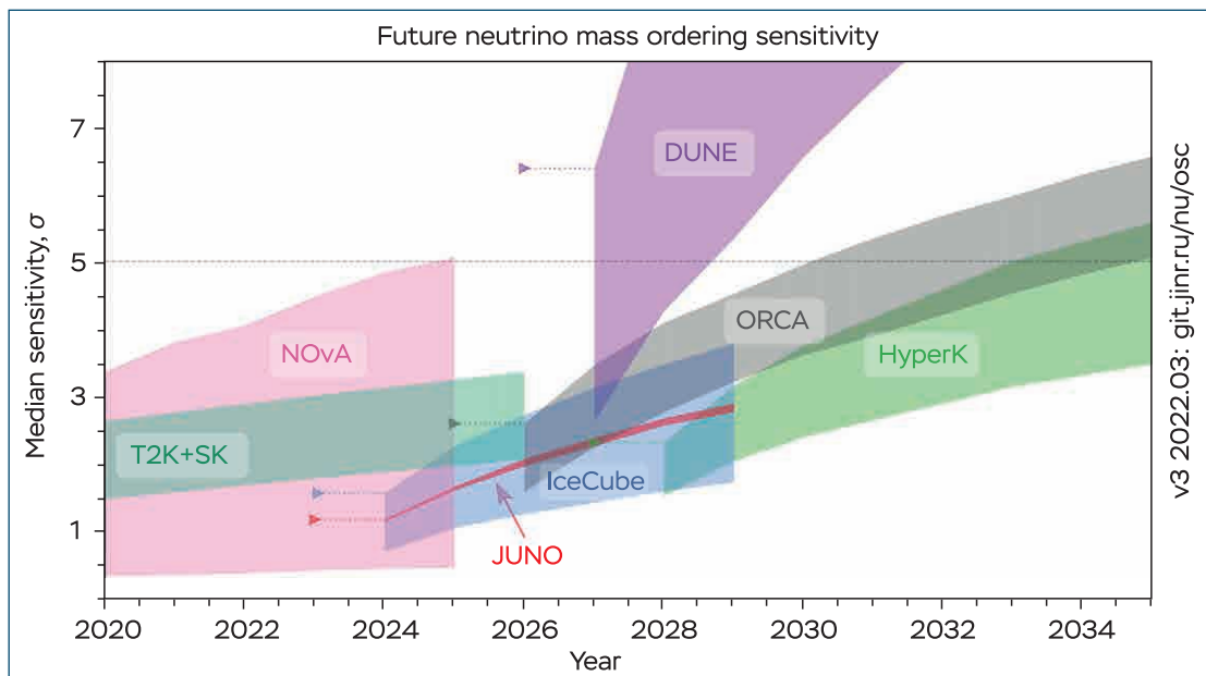
Fig. 18. Neutrino mass ordering sensitivity in current and planned experiments. The bands represent the entire range of possible measurements depending on other parameters
