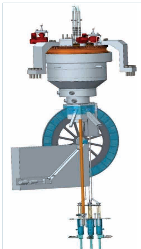
Fig. 8. A variant of the new NEPTUNE reactor
