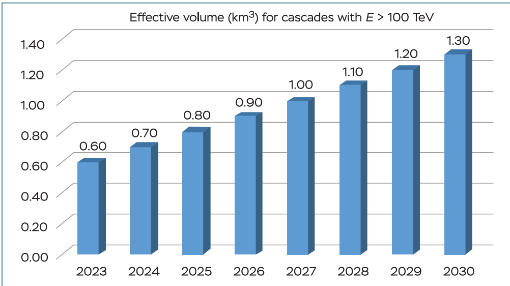
Fig. 11. The Baikal-GVD experiment. Detector expansion plan in terms of effective volume in the problem of astrophysical flow detection
