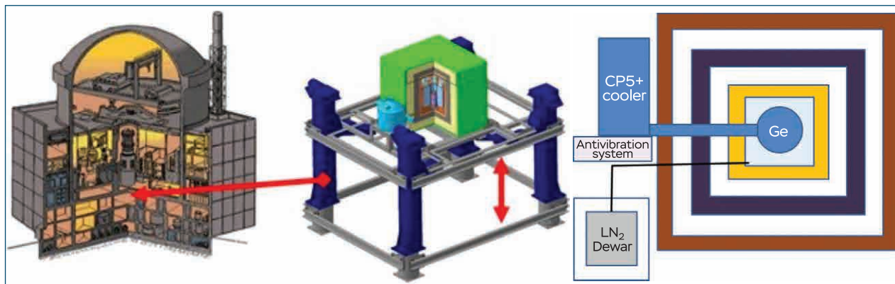
Fig. 19. Scheme of the \nu GeN setup aimed at detecting CEvNS. The setup is located directly under the Kalinin Nuclear Power Plant reactor No.3 (left), on a special lifting device (centre) that allows changing the antineutrino flux in the HPGe detector, surrounded by a complex active and passive shielding (right)
