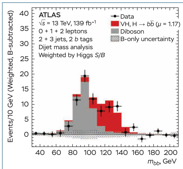
Fig. 15. The invariant mass distribution of a pair of b quarks obtained in pp collisions at an energy of 13 TeV in the ATLAS experiment in the processes of associated production of the Higgs boson with W and Z bosons and its decay into a pair of b quarks. The contribution from all background processes is subtracted, with the exception of WZ and ZZ
