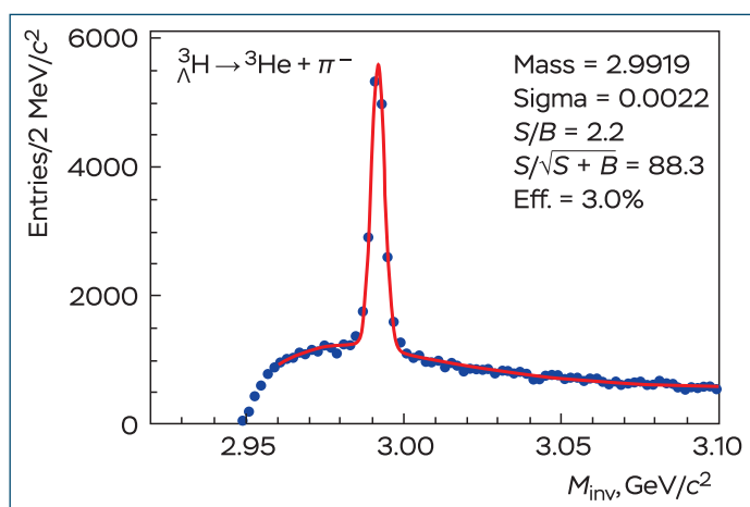
Fig. 14. To evaluate the prospects for studying hypernuclei at NICA, a detailed simulation of the MPD detector parameters was performed for the reconstruction of hypertritons in Bi+Bi collisions at a centre-of-mass energy of 9.2A GeV. The distribution of the reconstructed invariant mass of the hypertriton in two-body decay mode is shown for the statistics of 40 million Bi+Bi collisions
