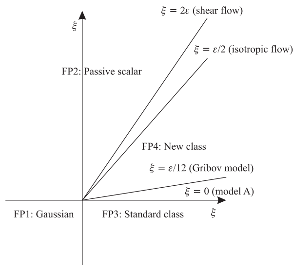
Regions of stability of the fixed points in various models
