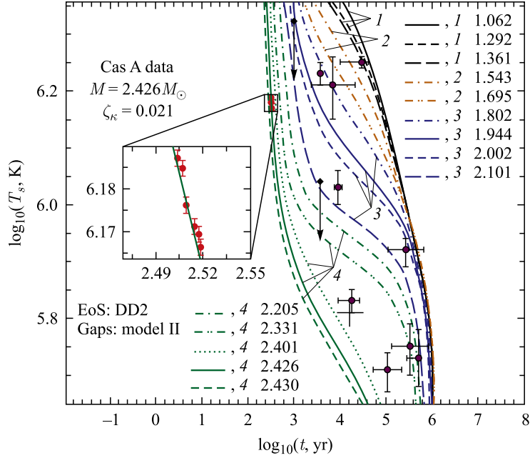
Fig. 2 (color online). Cooling curves for a neutron star sequence according to the stiff hadronic DD2 EoS; T_s is the surface temperature, t is the CS age. The color coding corresponds to different mass ranges: M = 1.0\text{--}1.5M_{\odot} (black, 1), M = 1.5\text{--}1.8M_{\odot} (orange, 2), M = 1.8\text{--}2.2M_{\odot} (blue 3) and M = 2.2\text{--}2.5M_{\odot} (green, 4). Cooling data for Cas A are explained with a heavy neutron star of M = 2.426M_{\odot} . To recover an appropriate slope of the curve, a pre-factor \zeta_{\kappa} = 0.021 is required
