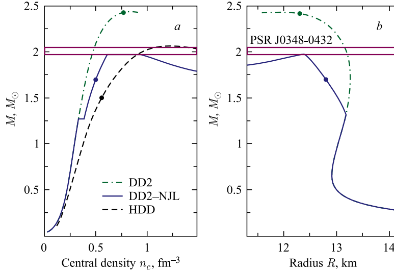
Fig. 1. Mass vs. central baryon density ( a ) and vs. radius ( b ) for the stiff DD2 hadronic EoS (dash-dotted lines) and for the hybrid EoS with a deconfinement transition to superconducting NJL quark matter (solid lines). For comparison, the softer hadronic EoS model HDD [17] is shown in panel a (dashed line). All three EoS fulfil the constraint for the maximum mass of 1.97M_{\odot} . The dots indicate the configurations for which the cooling curve would describe the observational data from Cas A
