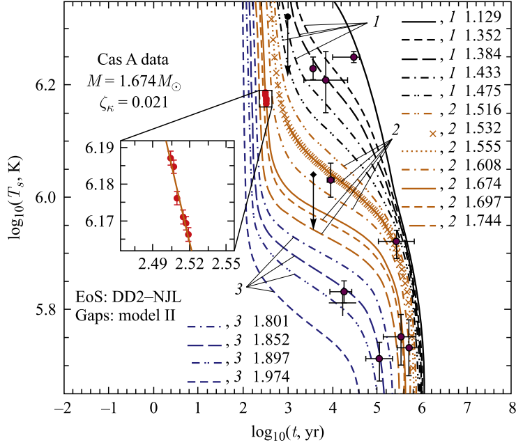
Fig. 3 (color online). Cooling curves for a CS sequence according to the DD2–NJL hybrid EoS. The color coding is as in Fig. 2. Cooling data for Cas A are explained with a quark core hybrid star of M = 1.674M_{\odot} . To recover an appropriate slope of the curve, one requires a pre-factor \zeta_{\kappa} = 0.021
