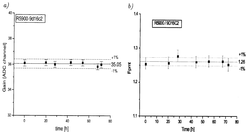
Fig. 6. The time stability of the PMT R5900/9d16c2 : a ) the PMT gain ( Q_1 ) vs time [hours], b ) the excess factor vs time (hours); the used light source intensity applied was \approx 2 photoelectrons.
