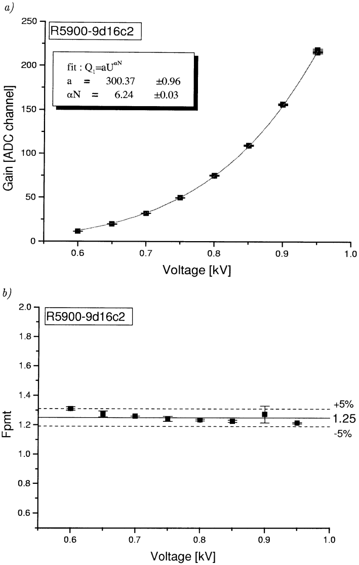
Fig. 5. The PMT R5900/9d16c2 characteristics: a ) dependence of the PMT gain ( Q_1 ) on voltage (kV), b ) dependence of the excess factor on voltage.
