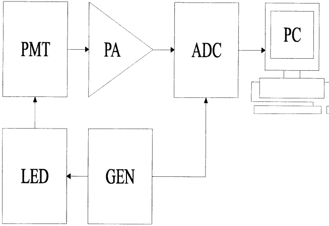
Fig. 1. Block scheme of the experimental setup for the measurement of single photoelectron spectra.
