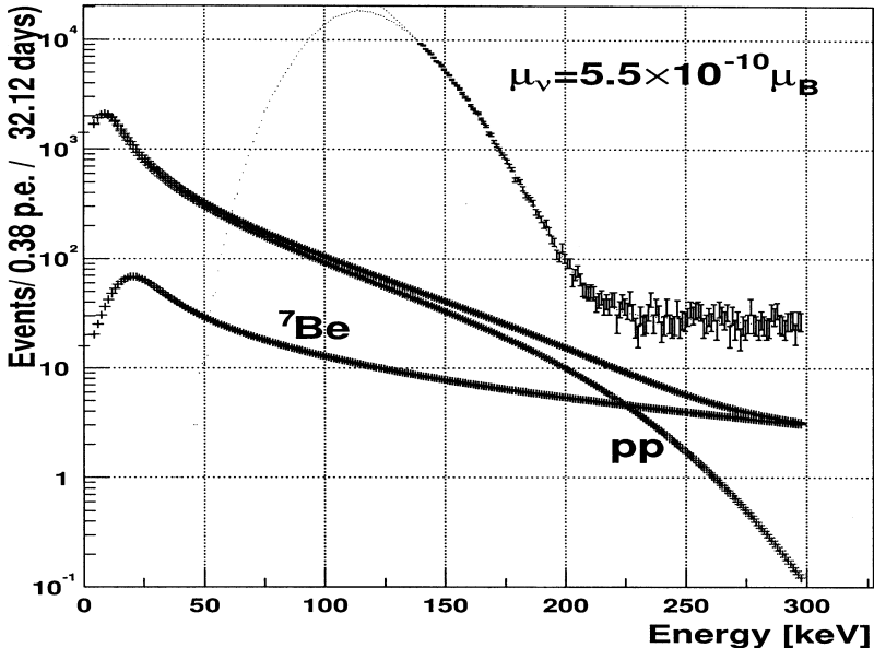
Figure 3: The experimental spectrum (upper plot with error bars) and the expected spectra for magnetic scattering of pp and {}^7\text{Be} neutrinos calculated in accordance with ( ) and ( ).
