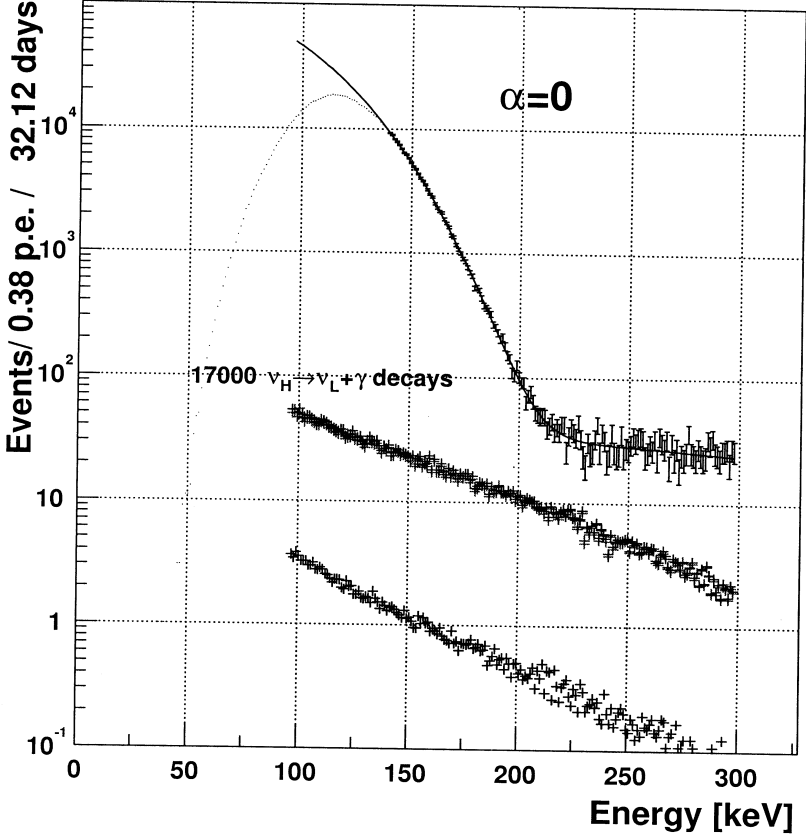
Figure 4: The results of fitting for \alpha = 0 . The experimental spectrum (upper plot with error bars) and the results of the Monte Carlo simulation of 17000 \nu_H \rightarrow \nu_L + \gamma decays in the scintillator are shown.
