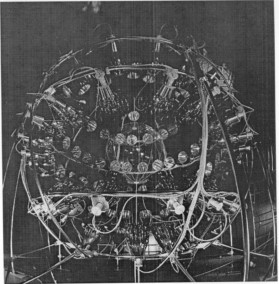
Figure 1: The view of the CTF detector
