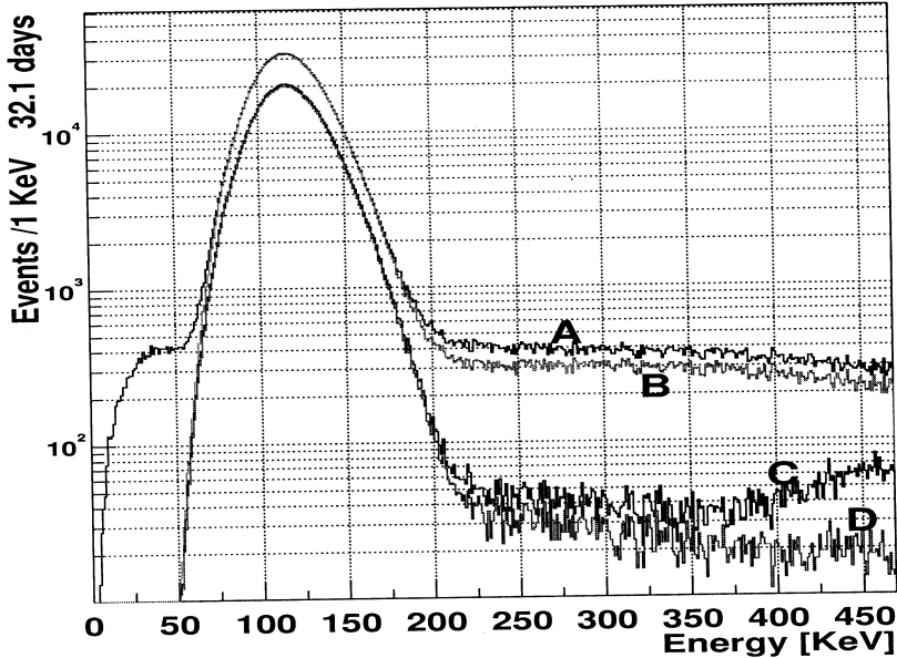
Figure 2: CTF-II background in the low energy region and the result of the sequential cuts applied in order to reduce background: A) raw data; B) muons cut; C) radial cut (with 100 cm radius); D) \alpha/\beta discrimination.
