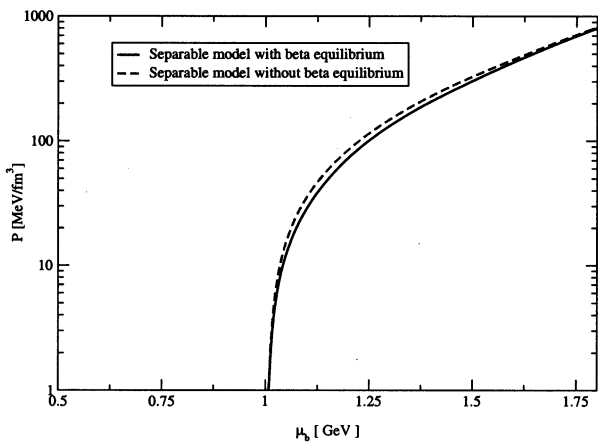
Figure 5 Pressure of three-flavor quark matter with \beta equilibrium and without.
