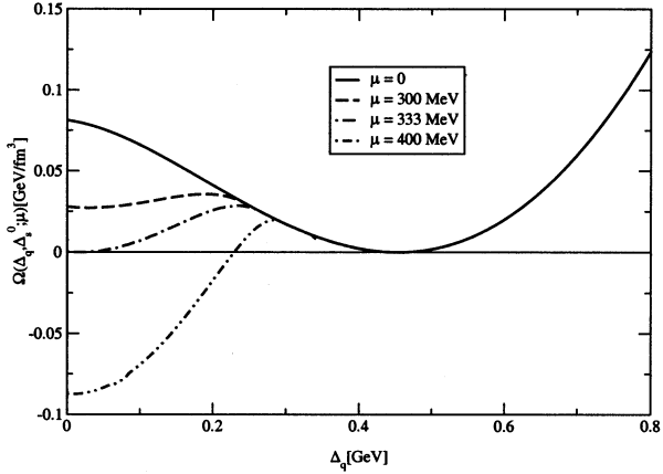
Figure 1 Dependence of the thermodynamical potential on the light flavor gap \Delta_q = \Delta_u = \Delta_d (order parameter) for different values of the chemical potential, \Delta_s = 682 MeV.
