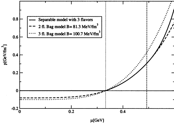
Figure 3 Pressure of the quark matter as a function of the chemical potential for the separable model (solid line) compared to a three-flavor (dotted line) and a two-flavor (dashed line) bag model. All models have the same critical chemical potential \mu_c = 333 MeV for (light) quark deconfinement.
