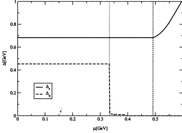
Figure 2 Solutions of the gap equations that minimize the potential
