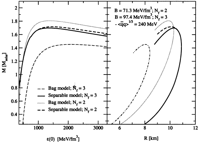
Figure 6 Stability for compact stars composed of quark matter.
