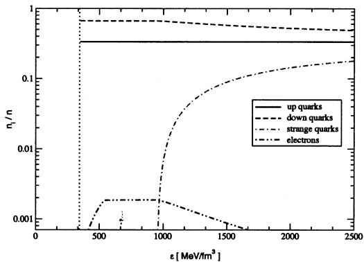
Figure 4 Composition of three-flavor quark matter in \beta equilibrium with electrons.
