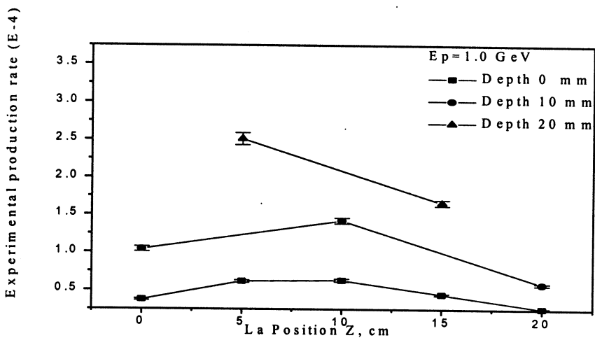
Fig. 5-b Experimental production rate for La sensors as a function of the sample position. Distances along Z axis are measured relative to the front plate of the lead target
