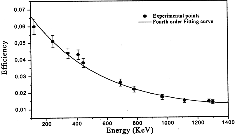
Fig.3 Efficiency curve for HPGGe detector used for measuring gamma rays in the decay of ^{140}\text{La} samples
