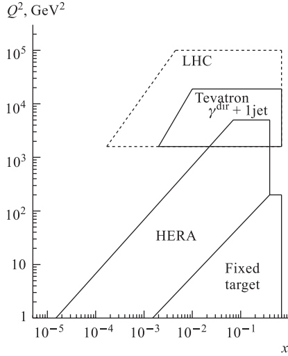
Fig. 2. Kinematic region for pp(\bar{p}) \rightarrow \gamma + \text{jet} + X process at Tevatron and LHC
