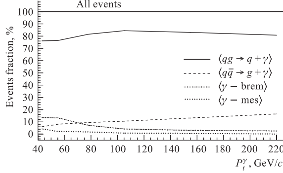
Fig. 1. The contributions of various event types to the total number of events as a function of P_t^\gamma
