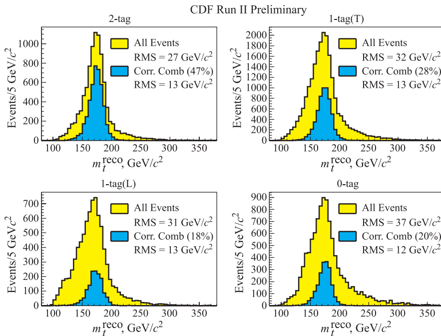
Fig. 2. Reconstructed top quark mass for 2-tag (top left), 1-tag(T) (top right), 1-tag(L) (bottom left) and 0-tag (bottom right) signal events ( M_{\text{top}} = 178 \text{ GeV}/c^2 , \text{JES} = 0 )
