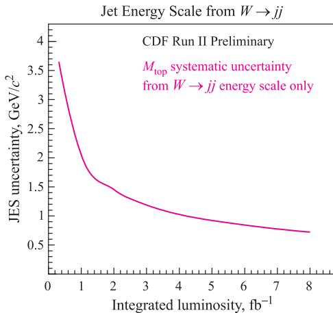
Fig. 12. Jet energy scale uncertainty from W \rightarrow jj calibration only as a function of integrated luminosity
