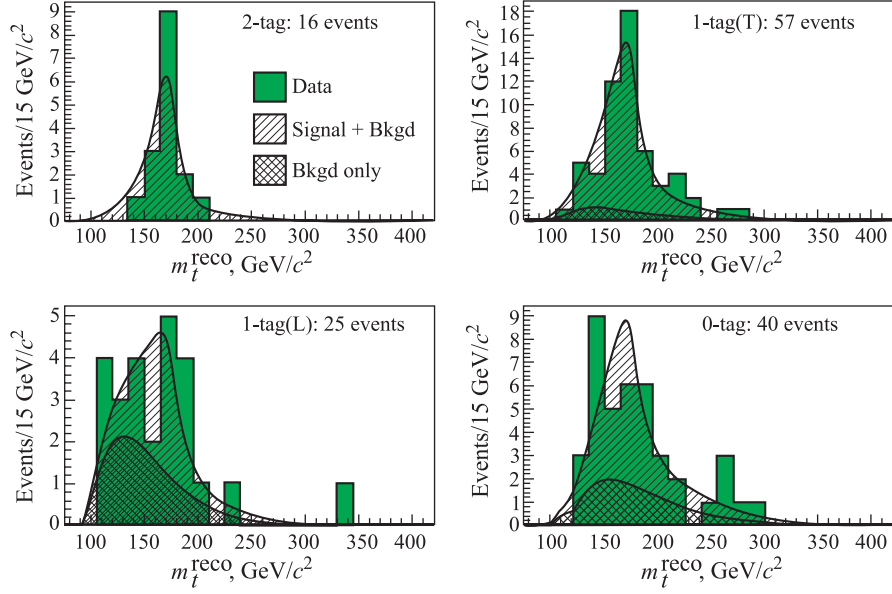
Fig.9. The reconstructed top quark mass distribution for each subsample is shown overlaid with the expected distribution using the top mass, jet energy scale, signal normalization, and background normalization from the combined fit
