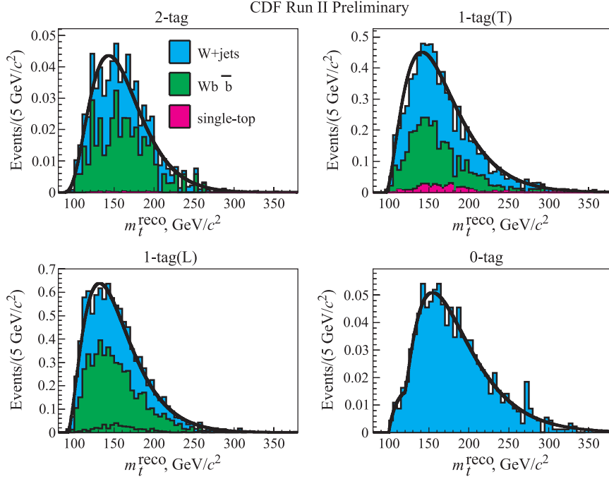
Fig. 5. Combined background m_t^{\text{reco}} templates for 2-tag events (top-left), 1-tag(T) events (top-right), 1-tag(L) events (bottom-left) and 0-tag events (bottom-right)
