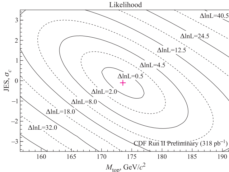
Fig. 8. The contours of the likelihood in the M_{\text{top}} - \text{JES} plane for the combined fit to all four subsamples. At each point in the plane, the likelihood is maximized with respect to the other free parameters. The cross-hair shows the best fit point
