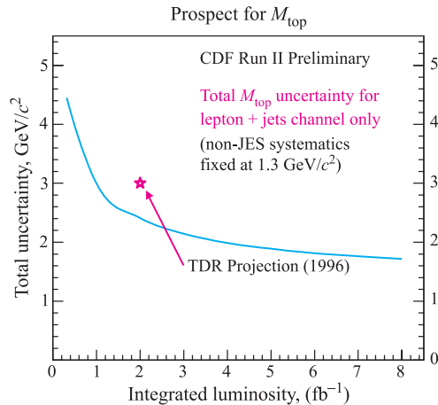
Fig. 13. Total M_{top} uncertainty as a function of integrated luminosity where the systematic uncertainties apart from JES are constant and equal to the current estimate. The projection of the CDF-II Technical Design Report [3] is indicated by a star
