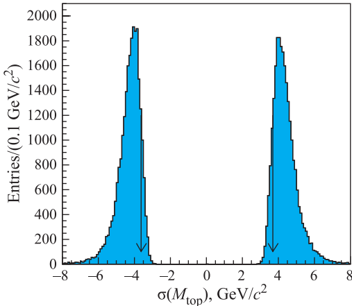
Fig. 11. The distributions of positive and negative uncertainties from the likelihood fit are shown, for pseudo-experiments generated with a true top mass of 172.5 \text{ GeV}/c^2 , the nominal jet energy scale, and the number of events in each subsample as observed in the data. Arrows indicate the positive and negative uncertainties from the likelihood fit to the data
