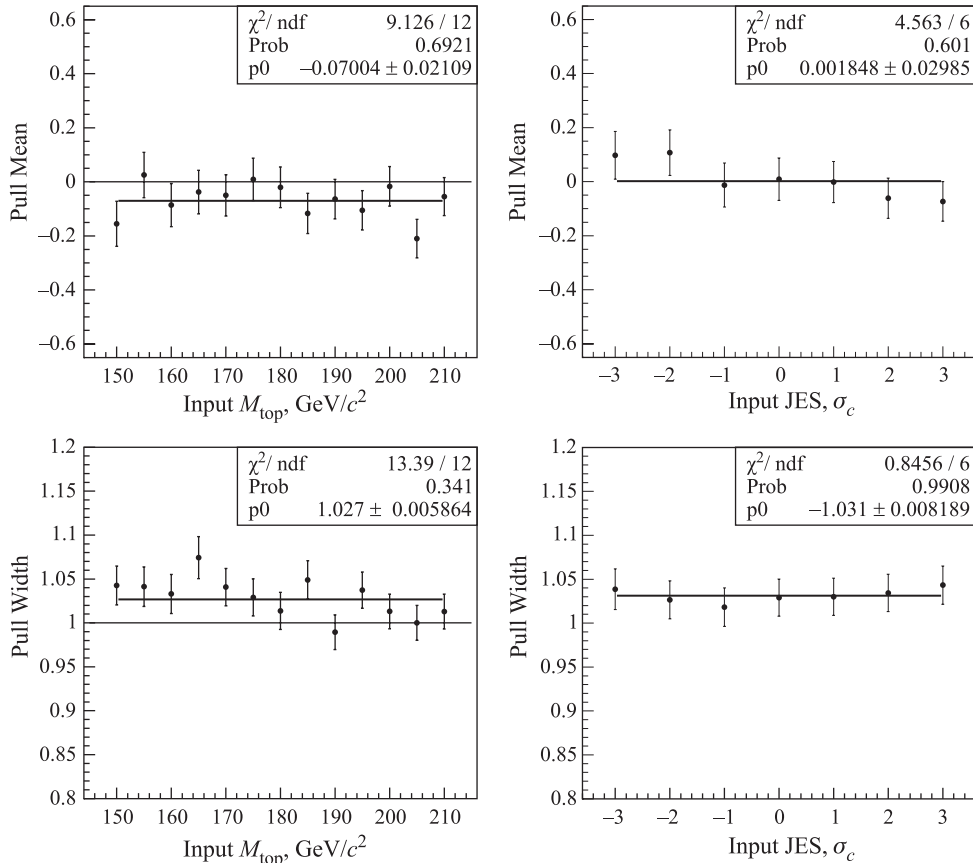
Fig. 7. The mean (top) and width (bottom) of pull distributions from sets of 2500 pseudo-experiments are shown. On the left, the jet energy scale is fixed at its nominal value, and the generated top quark mass is varied from 150 \text{GeV}/c^2 to 210 \text{GeV}/c^2 . On the right, the top quark mass is fixed at 175 \text{GeV}/c^2 , and the input jet energy scale is varied from -3\sigma to +3\sigma . The error bars come mostly from the limited statistics of the Monte Carlo samples from which the pseudo-data is taken
