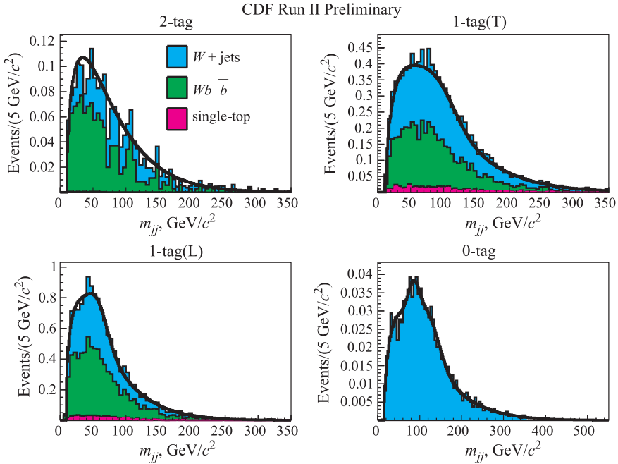
Fig. 6. Combined background m_{jj} templates for 2-tag events (top-left), 1-tag(T) events (top-right), 1-tag(L) events (bottom-left) and 0-tag events (bottom-right)
