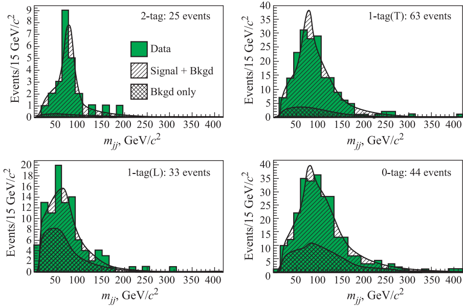
Fig. 10. The reconstructed dijet mass distribution for each subsample is shown overlaid with the expected distribution using the top mass, jet energy scale, signal normalization, and background normalization from the combined fit
