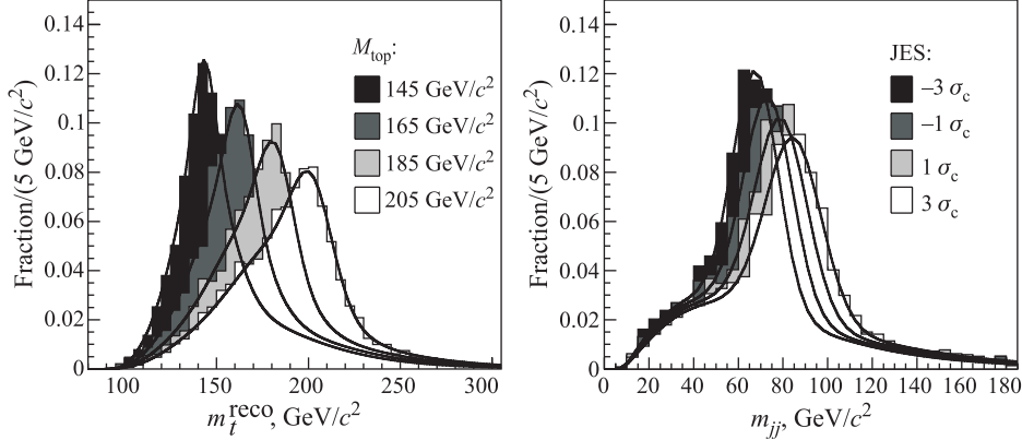
Fig. 4. Left plot: Signal m_t^{\text{reco}} templates are shown with top quark masses ranging from 145 \text{ GeV}/c^2 to 205 \text{ GeV}/c^2 and with JES set to 0 for the 1-tag(T) subsample. Right plot: Signal m_{jj} for JES values ranging from -3\sigma to +3\sigma , with M_{\text{top}} set to 175 \text{ GeV}/c^2 for the 2-tag subsample. Overlaid are the fitted parameterizations at each generated mass (left plot) and JES (right plot)
