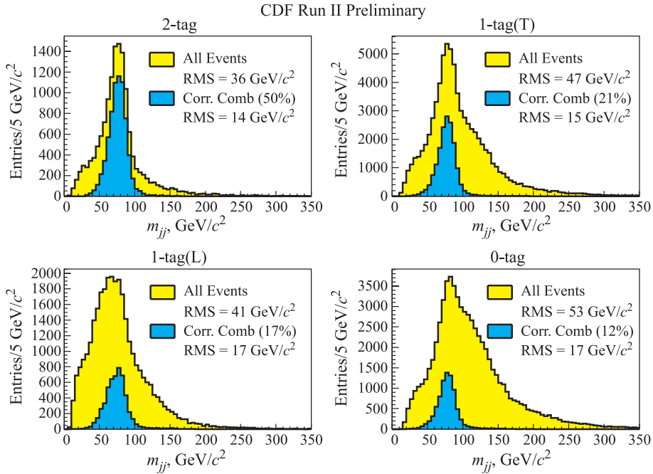
Fig. 3. Reconstructed hadronic W boson mass for 2-tag (top left), 1-tag(T) (top right), 1-tag(L) (bottom left) and 0-tag (bottom right) signal events ( M_{\text{top}} = 178 \text{ GeV}/c^2 , \text{JES} = 0 )
