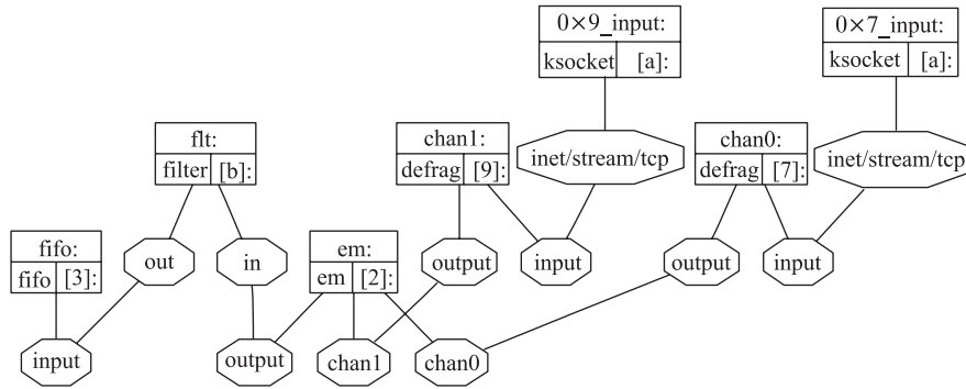
Fig. 2. A typical member of the SubEvB/EvB level is implemented by the ngdp graph. Legend the same as for Fig. 1. ng_em has two input channels ( chan0 and chan1 ) from two data sources (for example, two crate controllers) on FEM level (see Fig. 1). To simplify the picture, the ng_fifo outputs are not shown (see Fig. 1 for the typical ones).
