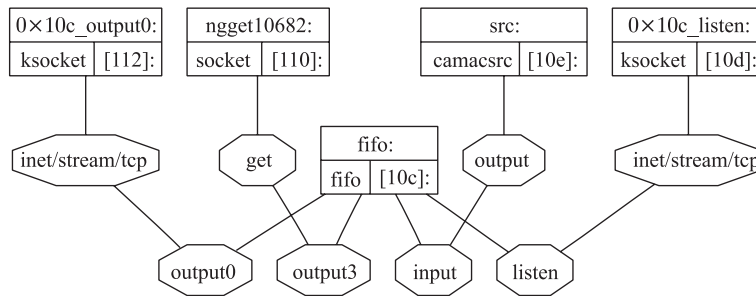
Fig. 1. A typical member of the CAMAC FEM level is realized by the ngdp graph. Rectangles are nodes with: name (up), type (left), ID (right). Octagons are nodes within. ng_fifo has two output streams — remote through accept()ing ng_ksocket and local through ng_socket — as well as listen()ing ng_ksocket
