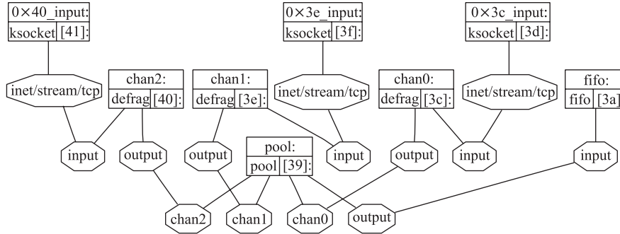
Fig. 3. A typical member of the pool level is implemented by the ngdp graph. Legend the same as for Fig. 1. ng_pool has three input channels ( chan0 , chan1 , chan2 ) from three data sources on EvB level (see Fig. 2). To simplify the picture, the ng_fifo outputs are not shown (see Fig. 1 for the typical ones).
