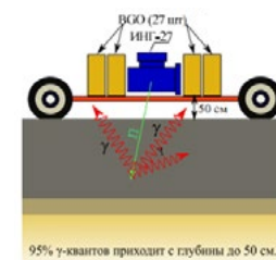
Sketch of the measuring setup
