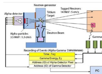
The TANGRA experimental setup
