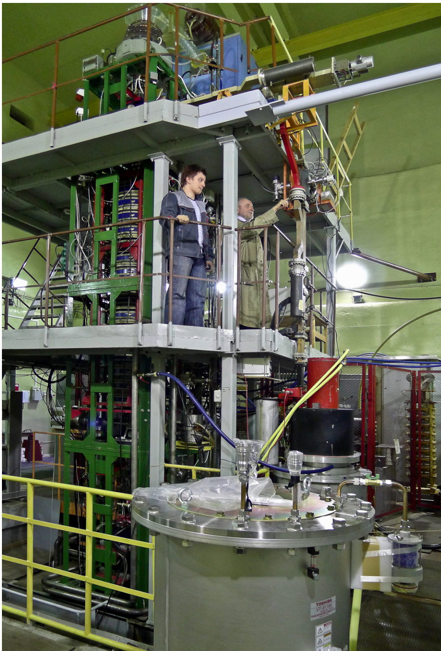
IREN – a new generation basic facility for research in nuclear physics
