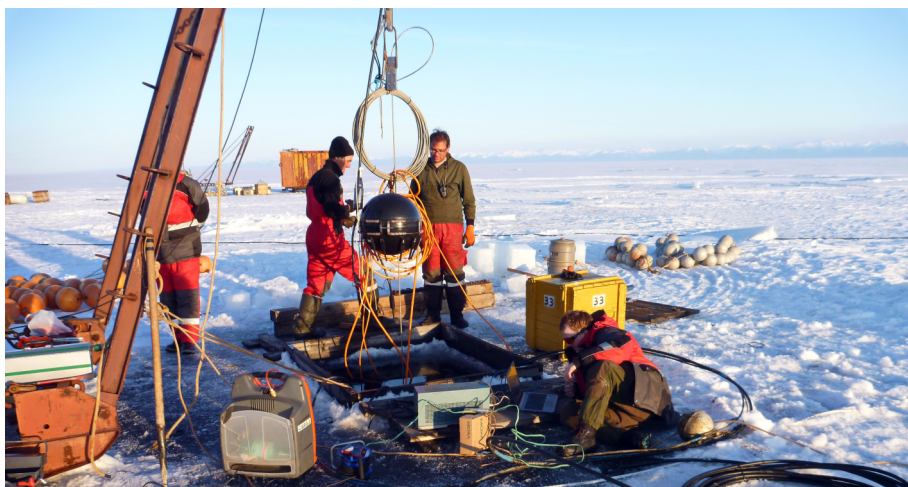
Assembling a string of optical modules for the Baikal-GVD neutrino telescope
