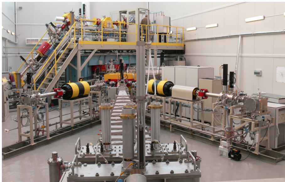
The DC-60 cyclotron developed at JINR for the Interdisciplinary Scientific Research Complex (ISRC) in Astana, Kazakhstan
