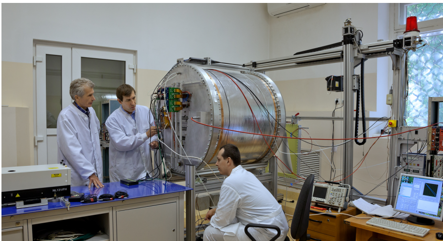
The Prototype of the time projection chamber TPC for the MPD NICA
