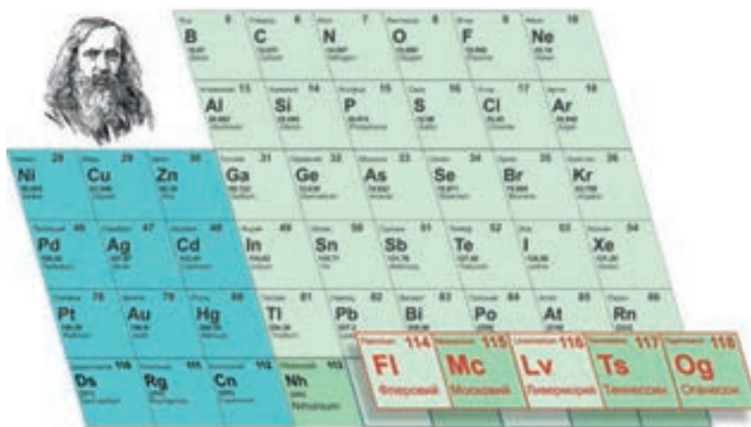
Part of D. I. Mendeleev's Periodic Table
