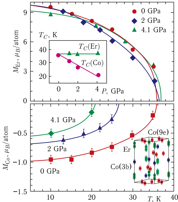
Temperature dependence of the magnetization of Er and Co sublattices in \text{ErCo}_2 at different pressures illustrating their independent behavior. The inserts show pressure dependences of Curie temperatures of Er and Co sublattices and the nature of the magnetic ordering in these compounds
