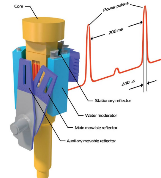
Schematic representation of the IBR-2 Reactor's operation
