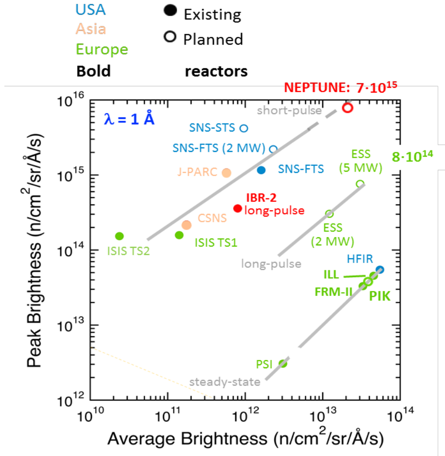
Fig. 9. Pulsed and average brightness for thermal neutrons of the IBR-2 reactor and the developed NEPTUNE source in comparison with neutron sources of various neutron centers
