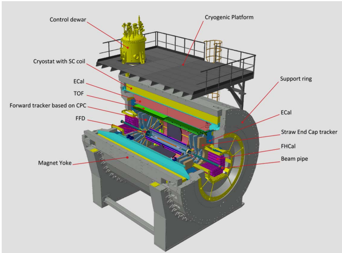
Fig. 4. General scheme of the Multi-Purpose Detector (MPD)
