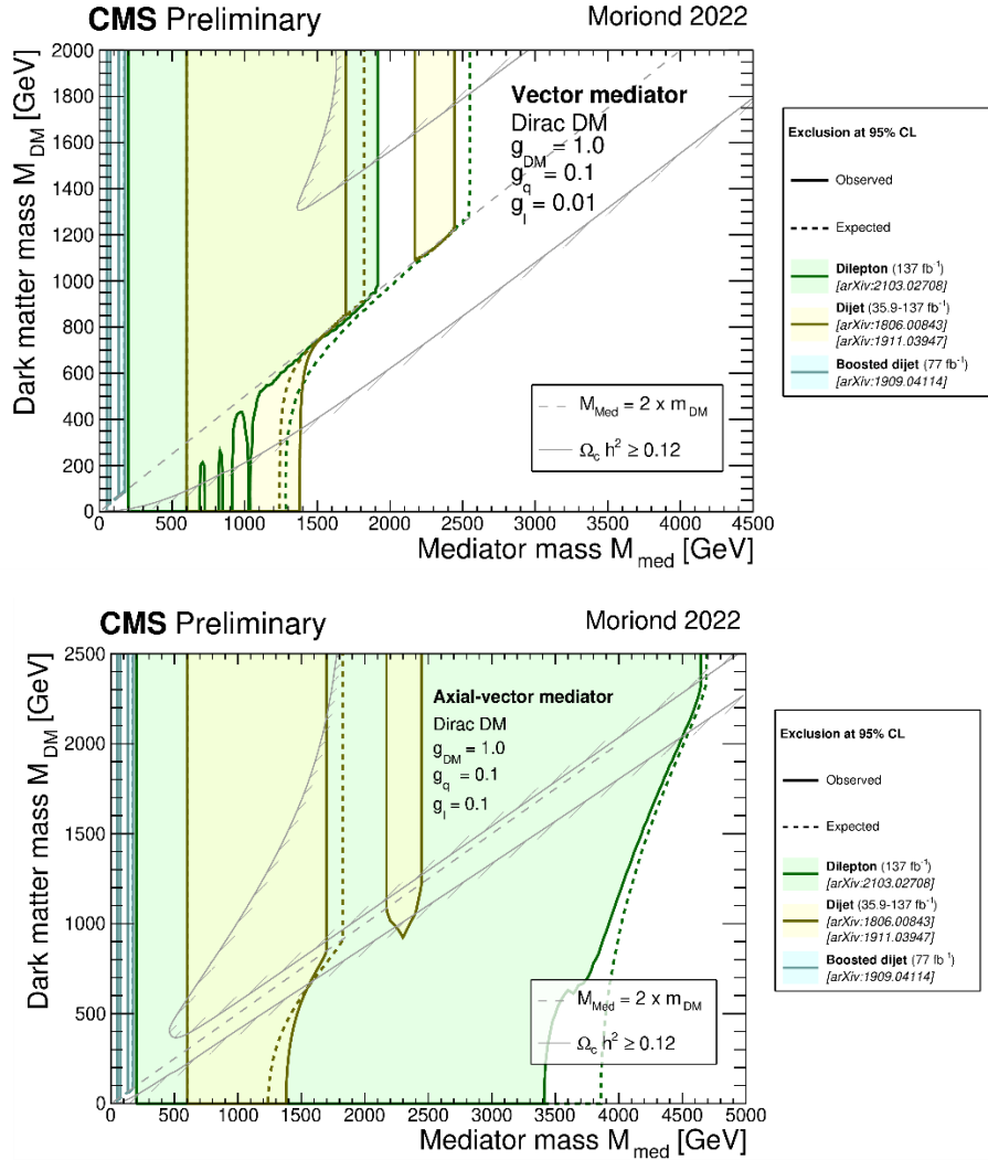
Рис. 15. In the combined channel of the production of a pair of jets and a pair of leptons in the events obtained in the CMS experiment at the LHC, the limits (95% C.L.) were determined on the masses of particle candidates for the role of dark matter particle m_{DM} and the mediator M_{med} . The shaded area corresponds to the excluded mass values for the vector (top) and pseudo-vector (bottom) mediator
