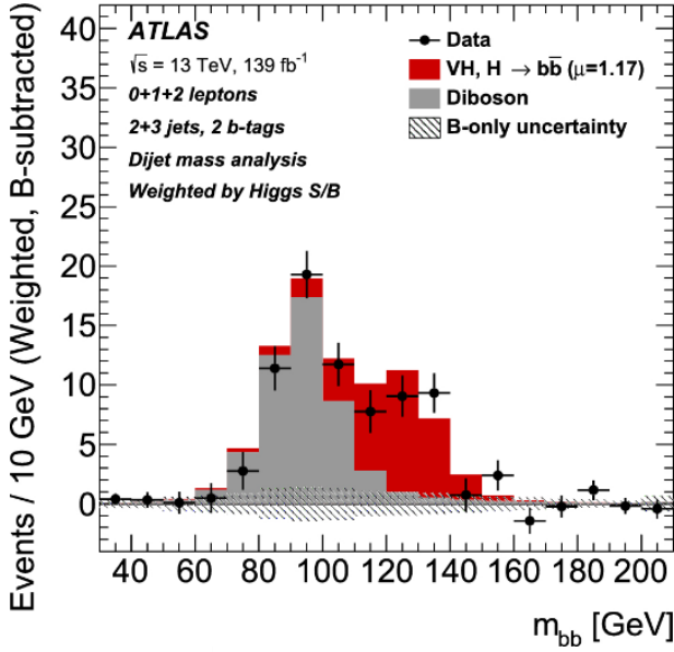
Рис. 14. The invariant mass distribution of a pair of b-jets obtained in pp collisions at an energy of 13 TeV in the ATLAS experiment in the processes of associated production of the Higgs boson with W and Z bosons and its decay into a pair of b-quarks. The contribution from all background processes is subtracted, with the exception of WZ and ZZ
